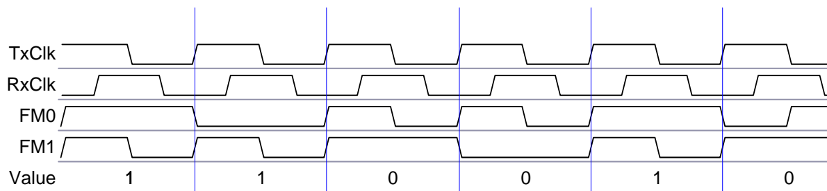
Figure 5 - FM0 and FM1 encoding
