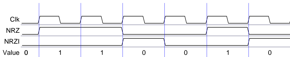
Figure 4 - NRZ and NRZI encoding
